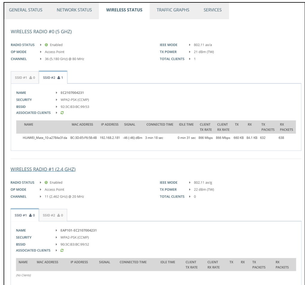
Figure 18: Wireless Status
