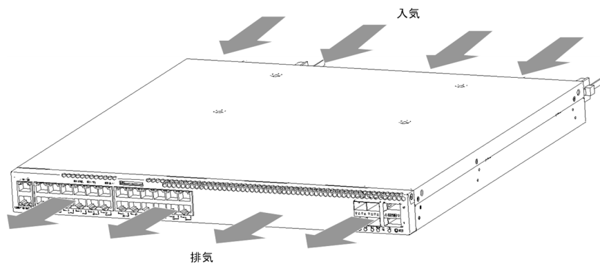
図2-8 AX3660S-24T4XW,AX3660S-48T4XW,AX3660S-16S4XW, AX3660S-24S8XW のエア フロー（背面吸気・前面排気構成時）
