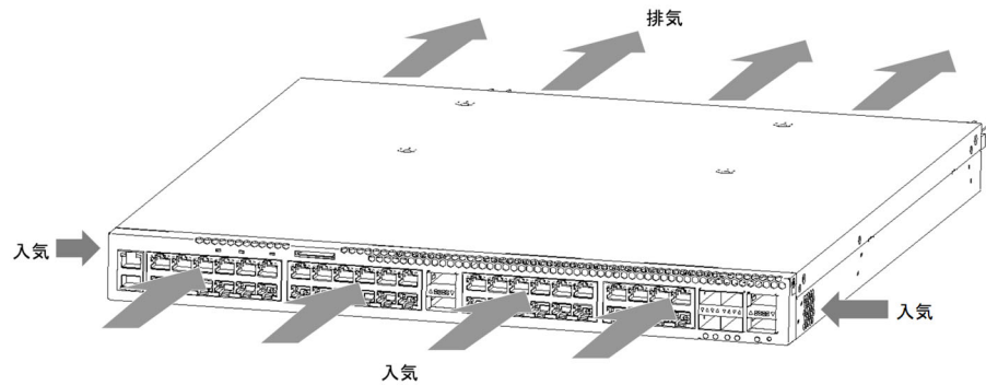
図2-9 AX3660S-48XT4QW, AX3660S-24X4QW, AX3660S-48X4QW のエアフロー（前面吸気・背面排気構成時）
