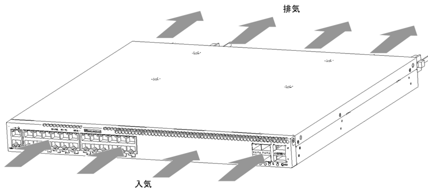
図2-7 AX3660S-24T4X,AX3660S-24T4XW,AX3660S-48T4XW,AX3660S-16S4XW, AX3660S-24S8XW のエアフロー（前面吸気・背面排気構成時）
