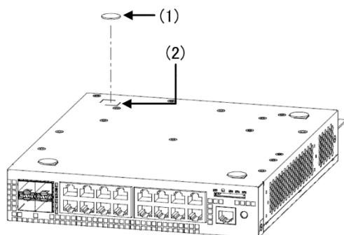
図 4-2 ゴム足の取り付け (AX2130S-16T, AX2130S-16P, AX2130S-24PH)
