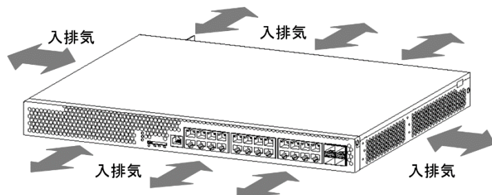
図 2-6 AX2230S-24T/AX2130S-24T/AX2130S-24TH/AX2130S-24PH/AX2130S-16T のエアフロー
