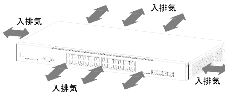
図 2-6 AX2230S-24T/AX2130S-24T/AX2130S-24TH/AX2130S-16T のエアフロー
