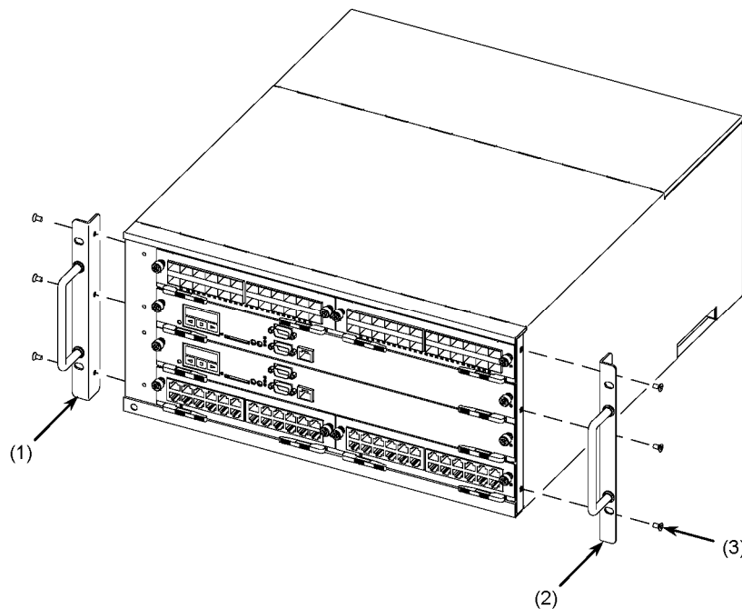
Figure 4-2 Removing the rack fixture
