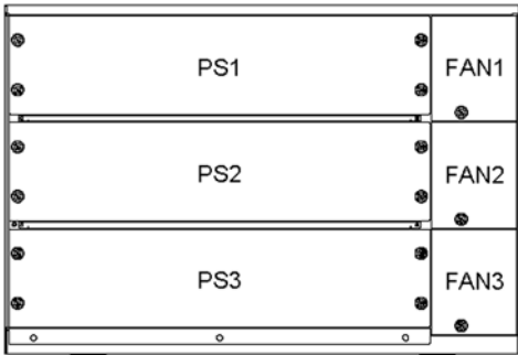
Figure 1-12 Rear of the Switch (with a DC power supply unit installed)
