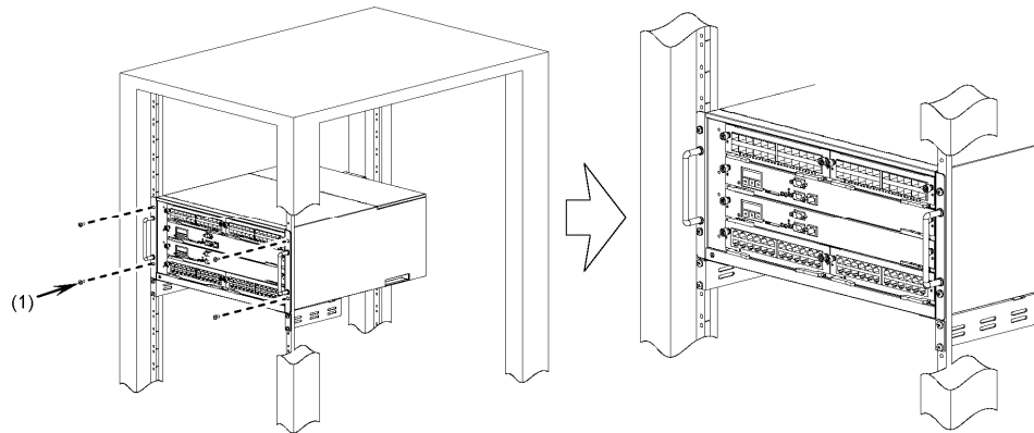
Figure 4-14 Securing the Switch
