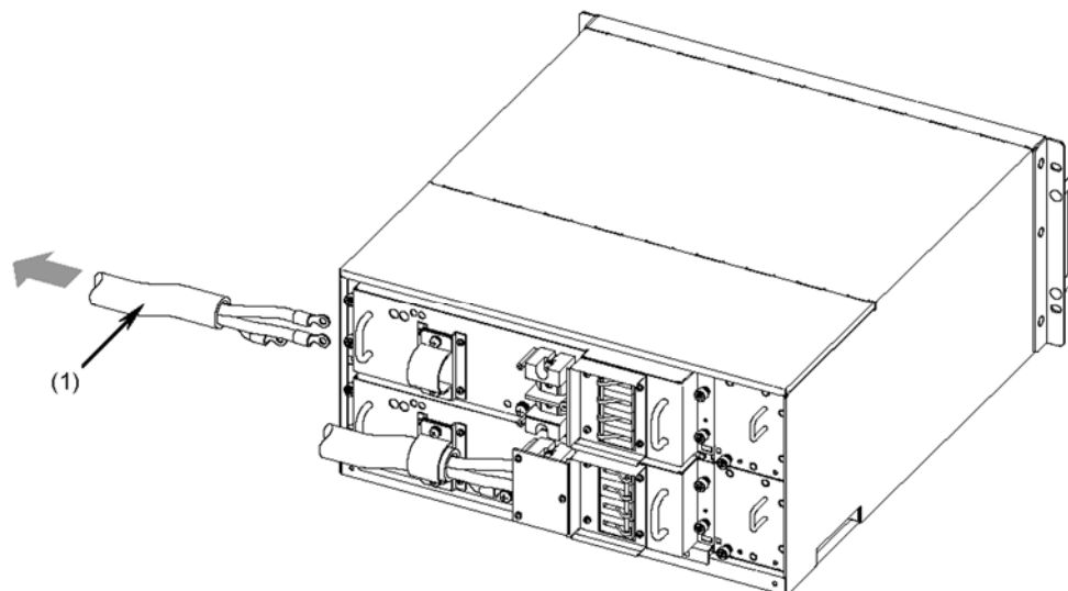
Figure 5-13 Disconnecting the power cable
