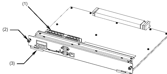
Figure 1-17 External appearance of the CSU-1A and the CSU-1B
