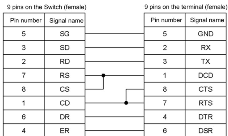
Figure 3-1 Connection cable for the operation terminal
