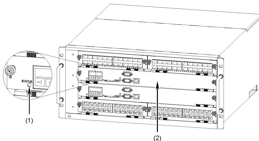
Figure 5-19 Checking the STATUS LED
