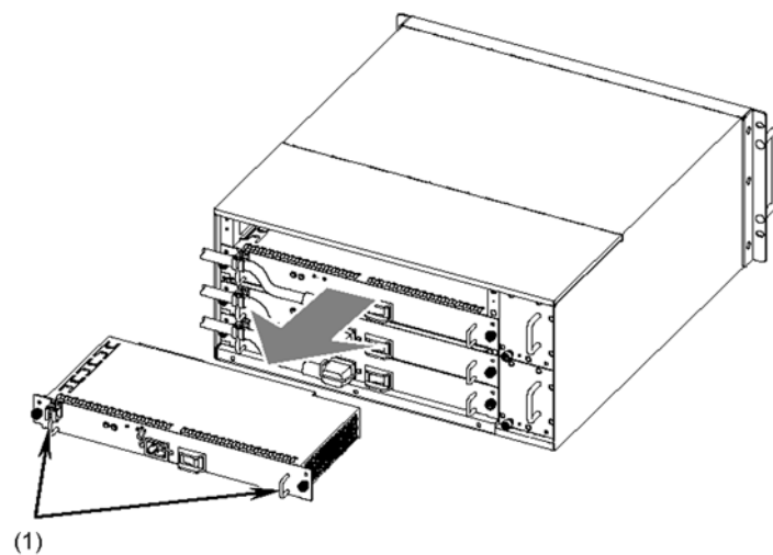
Figure 5-9 Removing a power supply unit (2)
