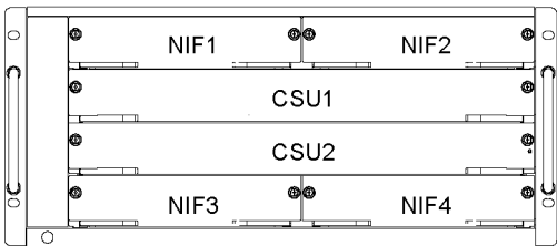
Figure 1-5 Rear of the Switch (with an AC power supply unit installed)
