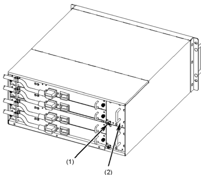
Figure 5-1 Removing a fan unit (1)
