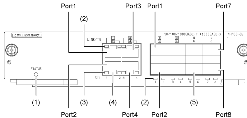
Figure 1-25 Front view
