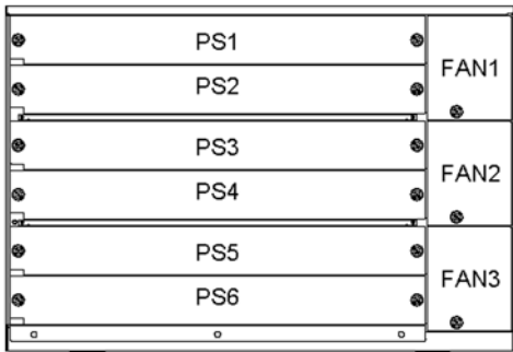
Figure 1-11 Rear of the Switch (with an AC power supply unit installed)
