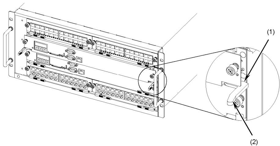
Figure 5-25 Installing a control and switching unit (2)
