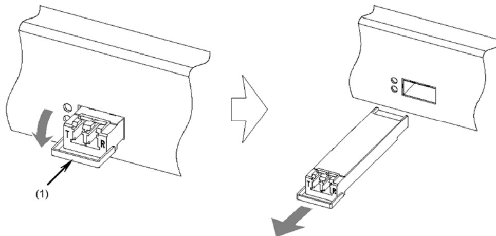
Figure 4-43 Removing an XFP transceiver
