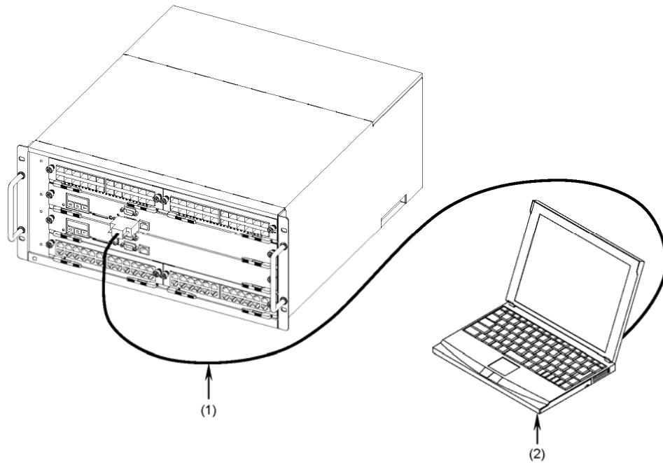
Figure 4-44 Connecting the operation terminal
