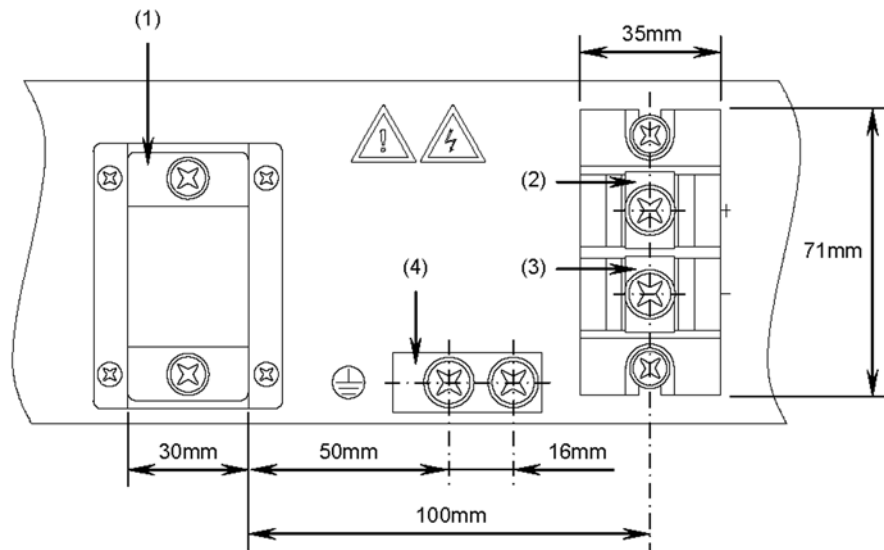
Figure 2-10 Terminal board of the DC power supply unit
