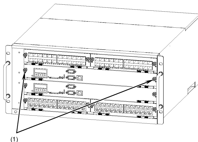
Figure 5-27 Installing a control and switching unit (4)
