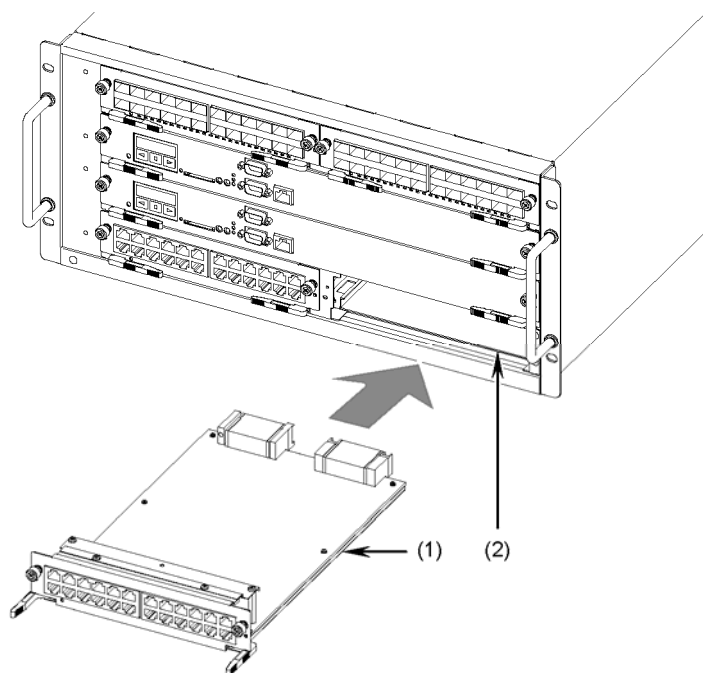
Figure 5-34 Installing a network interface unit (1)
