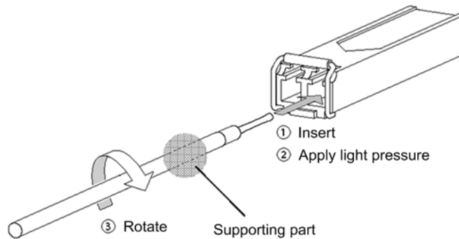
Figure A-3 Cleaning the ferrule tip
