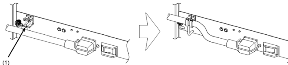
Figure 4-24 Clamping the power cable
