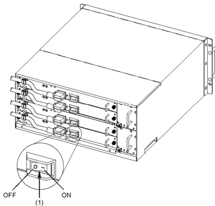
Figure 4-52 Turning off the power
