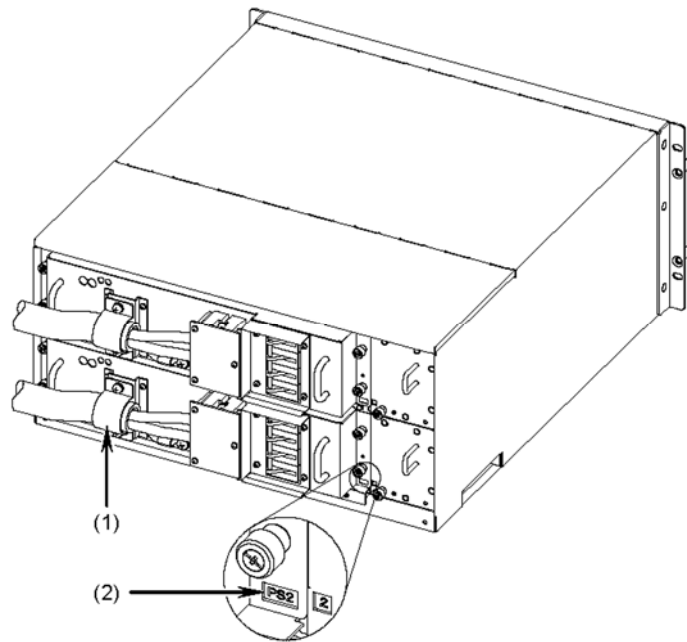
Figure 4-53 Checking the installation location of the power supply unit
