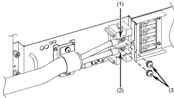
Figure 4-30 Securing the 0 V terminal and the -48 V terminal
