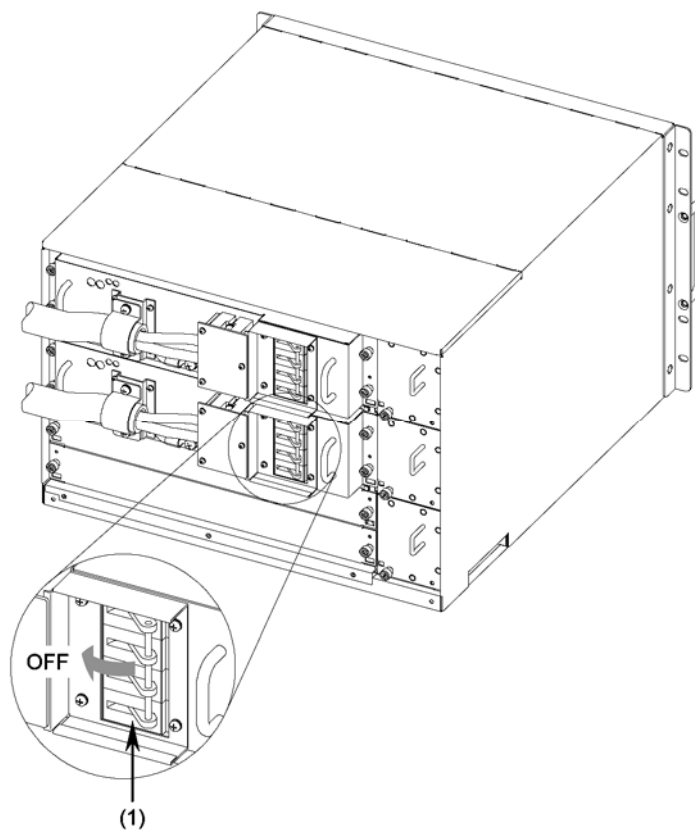
Figure 4-64 Turning off the power
