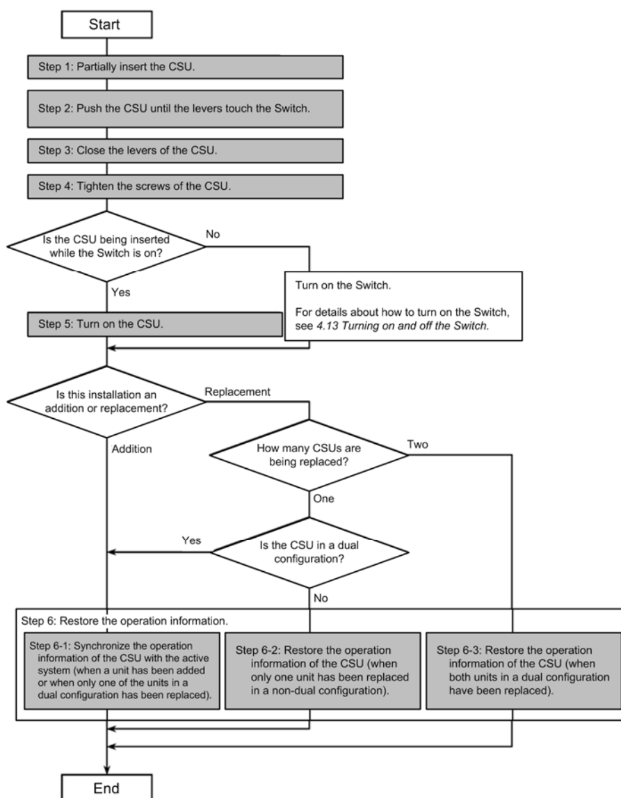
Figure 5-23 Installation overview
