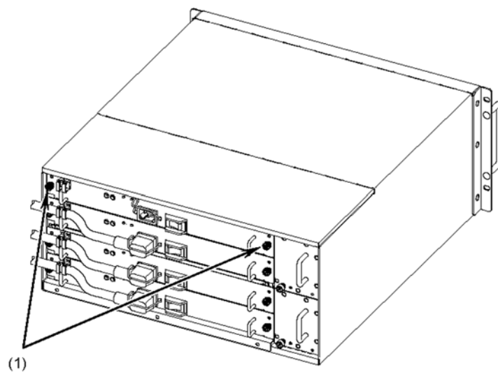
Figure 5-8 Removing a power supply unit (1)
