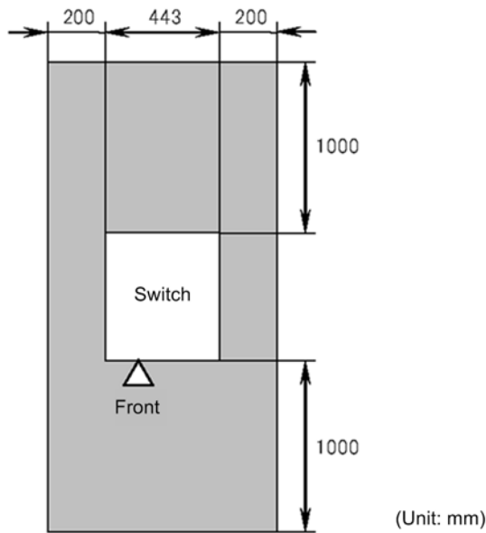
Figure 2-12 Maintenance area for a desktop installation
