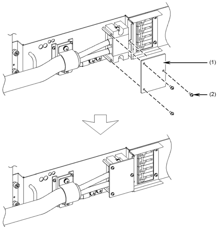
Figure 4-33 Attaching the terminal board cover
