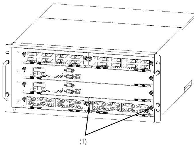
Figure 5-37 Installing a network interface unit (4)
