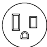
Figure 2-6 Two-pin grounded outlet (125V 15A)
