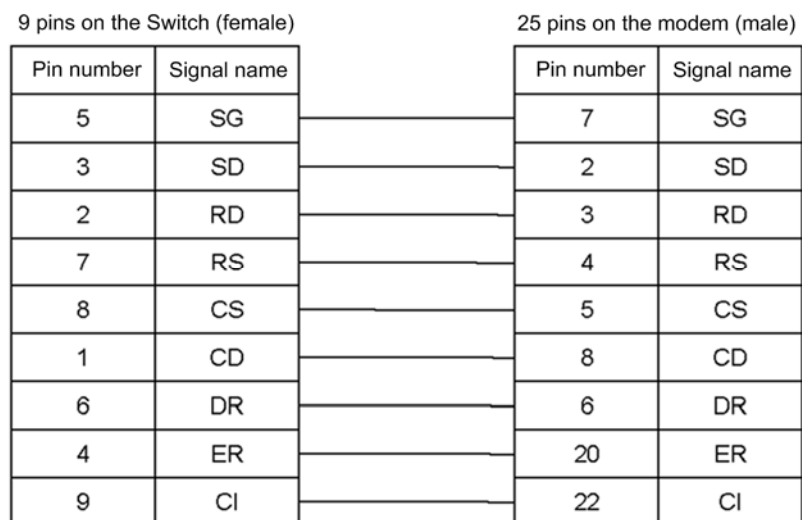
Figure 3-2 Modem connection cable
