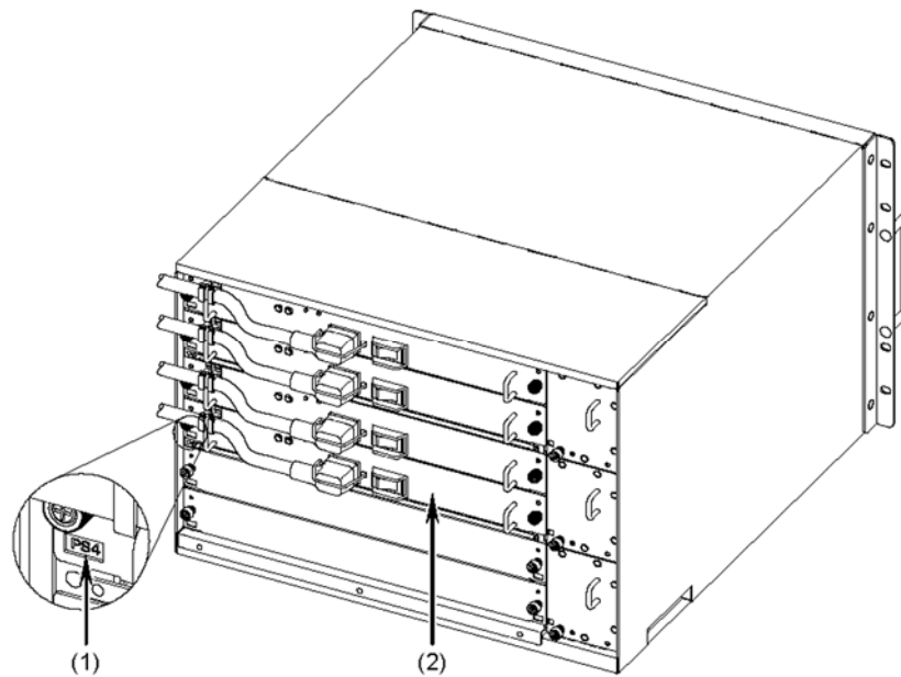
Figure 4-57 Checking the installation location of the power supply unit
