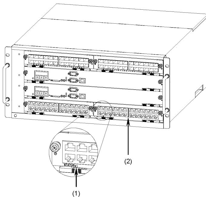
Figure 5-29 Checking the STATUS LED
