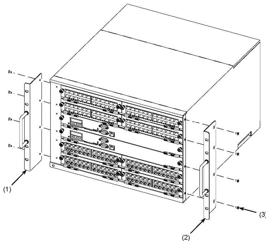
Figure 4-5 Attaching the rack fixture
