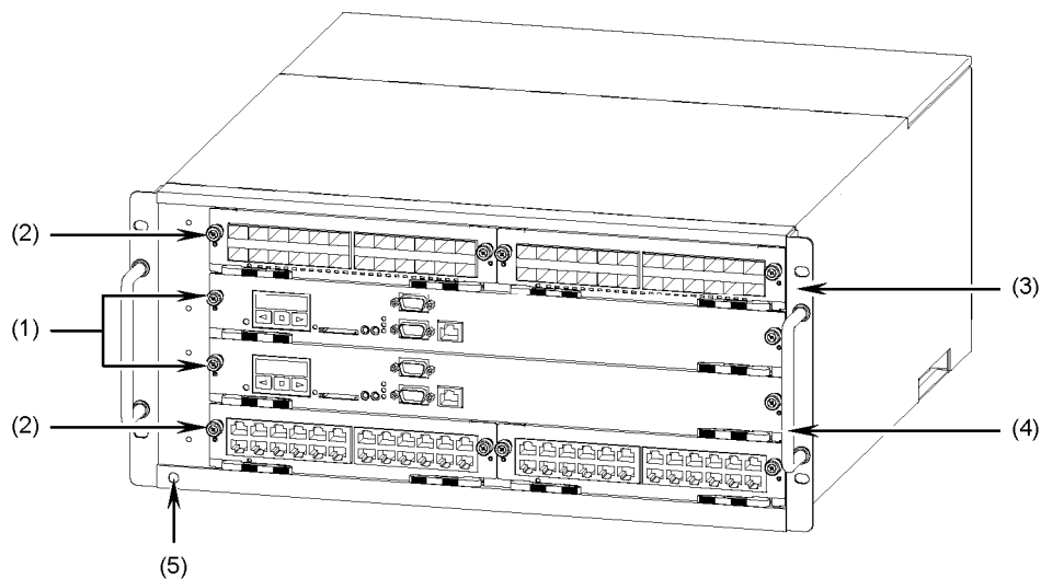
Figure 1-1 Front view
