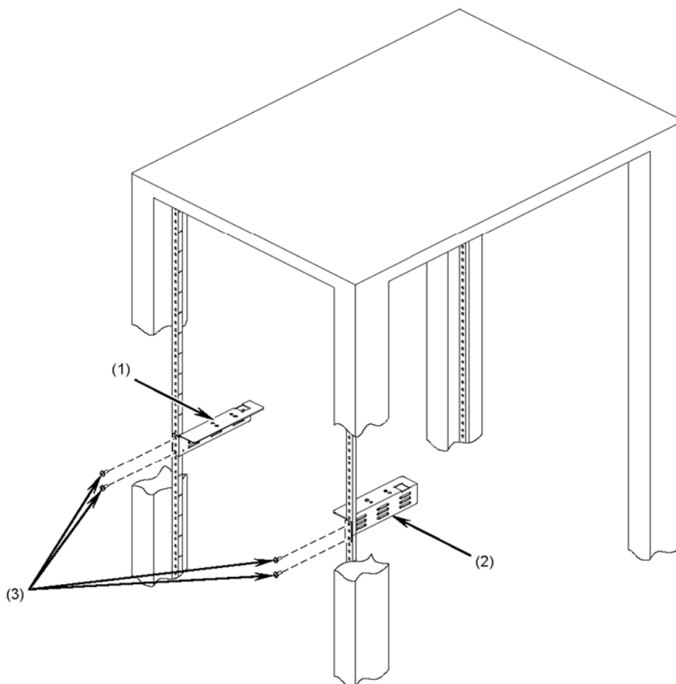
Figure 4-10 Installing support brackets
