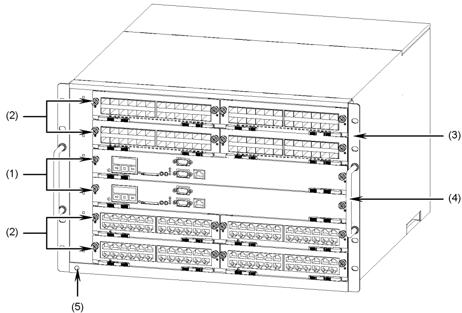
Figure 1-7 Front view
