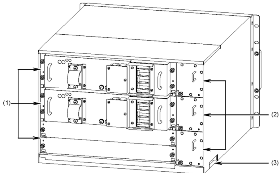
Figure 1-9 Rear view (with a DC power supply unit installed)
