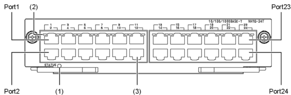
Figure 1-23 Front view
