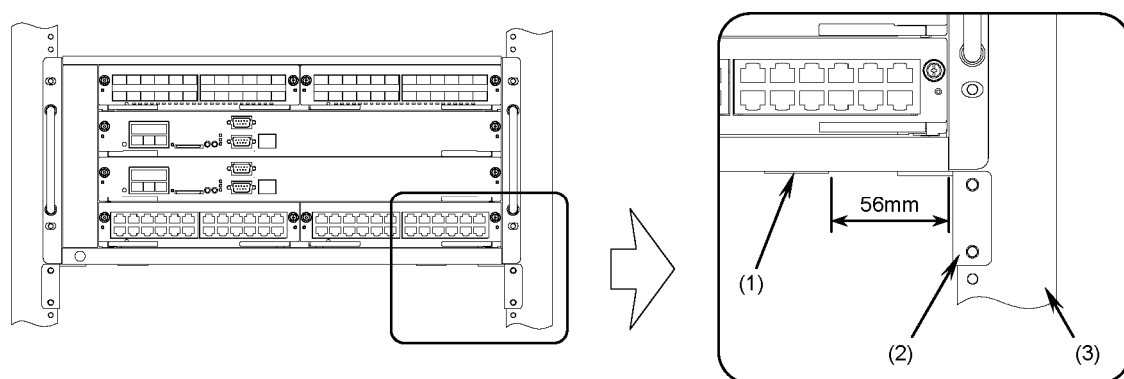
Figure 2-11 Guide rail details
