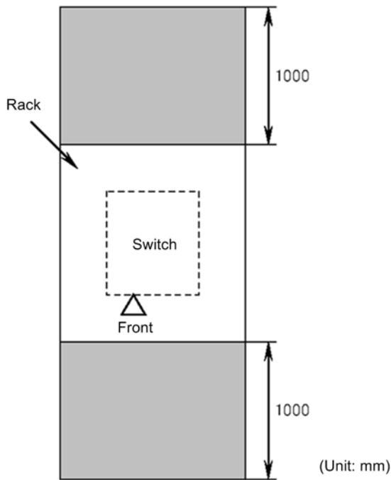
Figure 2-13 Maintenance area for a rack installation
