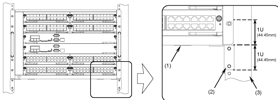
Figure 4-17 Installation location of the guide rail
