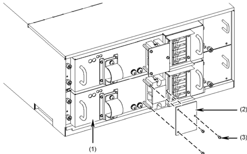
Figure 4-25 Removing the terminal board cover
