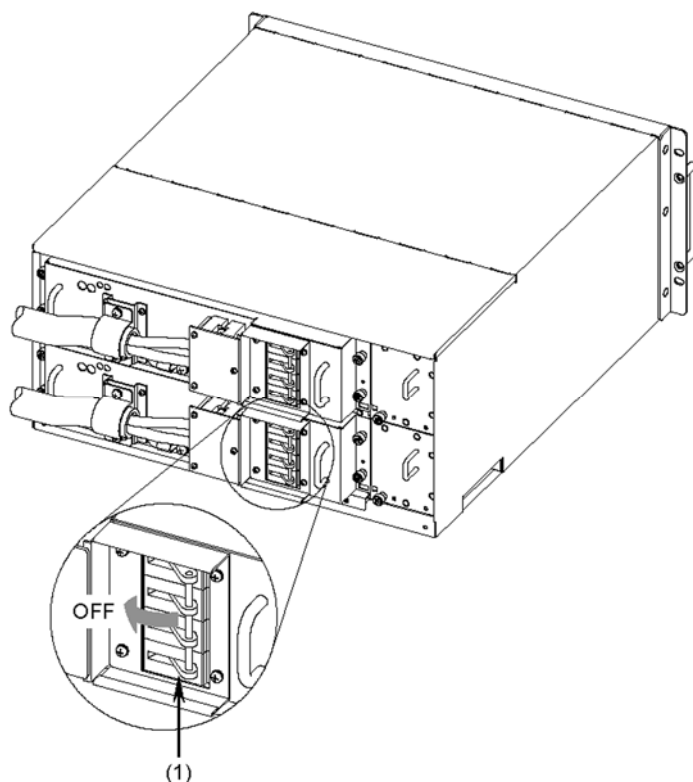
Figure 4-56 Turning off the power
