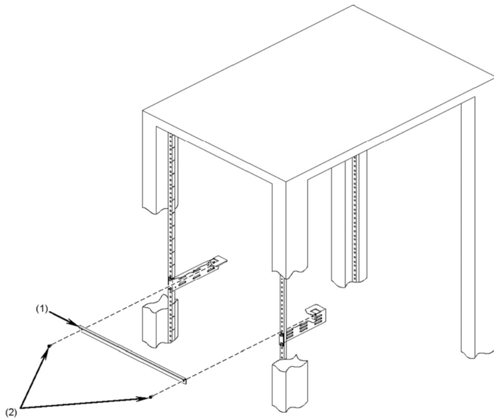
Figure 4-12 Attaching crossbar A
