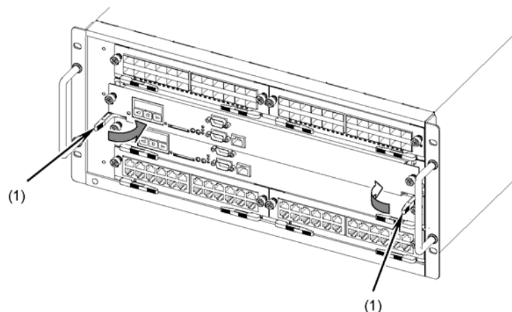
Figure 5-26 Installing a control and switching unit (3)
