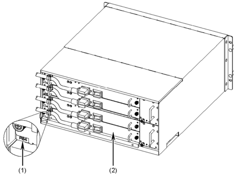
Figure 4-49 Checking the installation location of the power supply unit
