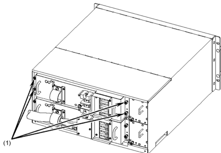
Figure 5-14 Removing a power supply unit (1)
