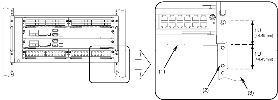
Figure 4-7 Installation location of the guide rail
