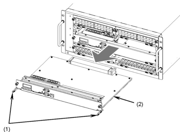
Figure 5-22 Removing a control and switching unit (3)
