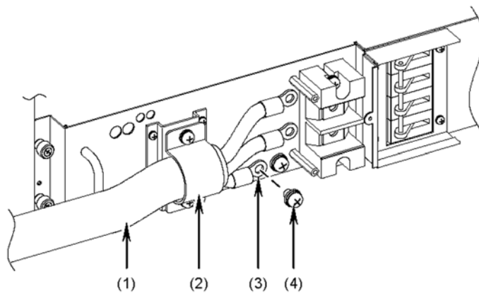
Figure 4-29 Securing the ground terminals
