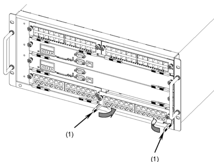
Figure 5-36 Installing a network interface unit (3)
