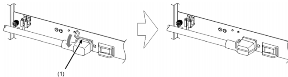
Figure 4-23 Clamping the power connector
