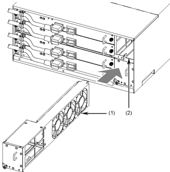
Figure 5-4 Installing a fan unit (1)
