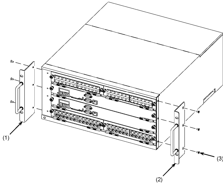
Figure 4-3 Attaching the rack fixture
