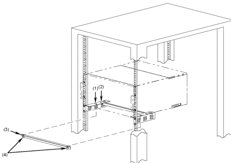
Figure 4-15 Attaching crossbar B
