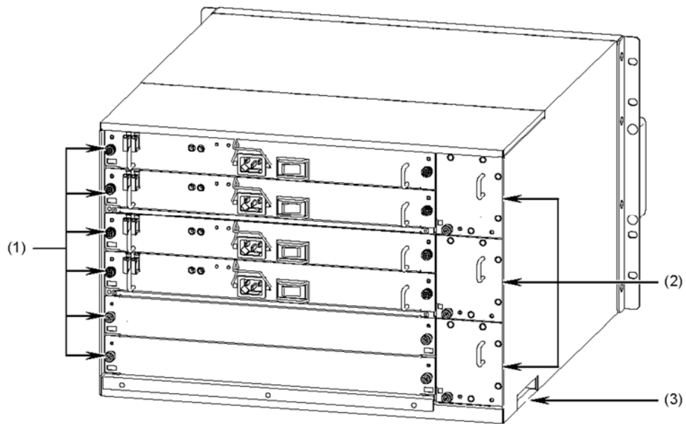
Figure 1-8 Rear view (with an AC power supply unit installed)
