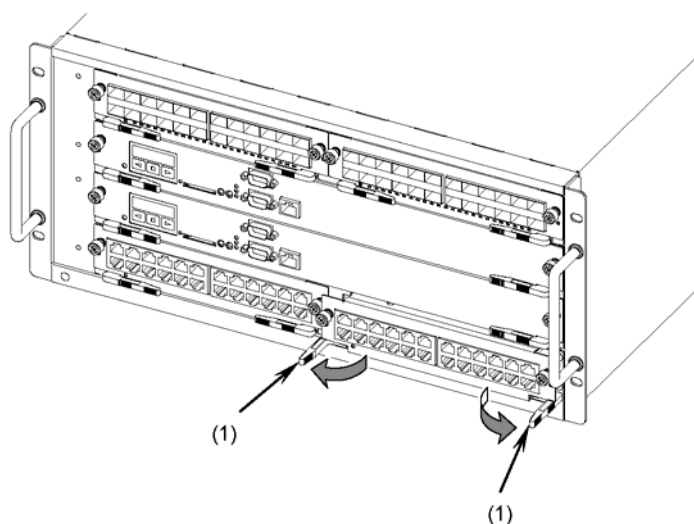
Figure 5-31 Removing a network interface unit (2)
