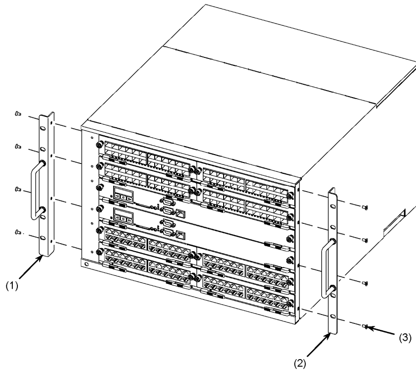
Figure 4-4 Removing the rack fixture
