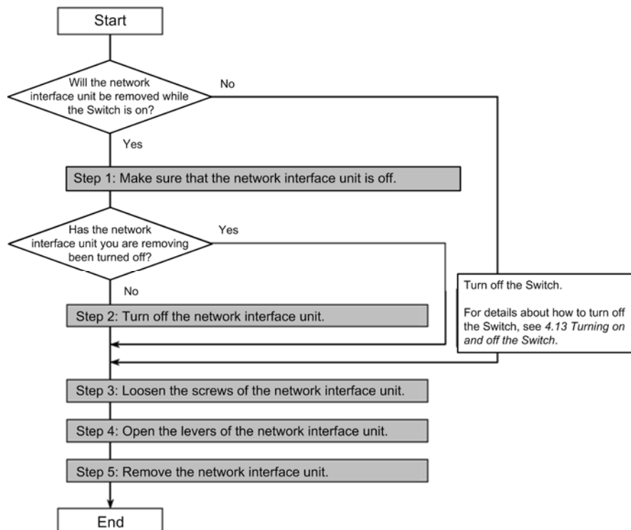
Figure 5-28 Overview of removing a network interface unit
