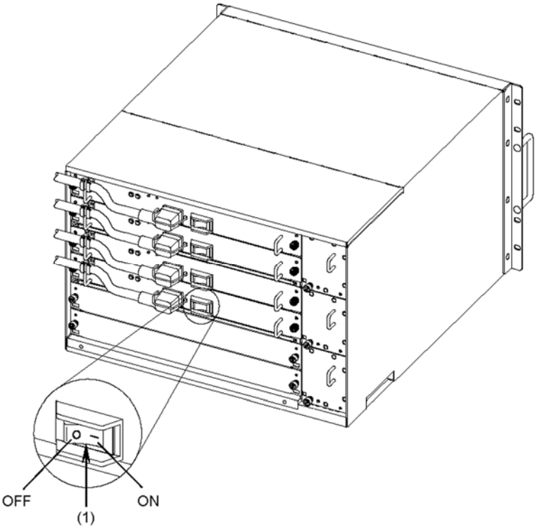
(1) Power switch
