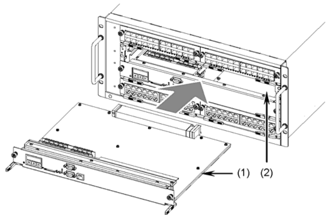
Figure 5-24 Installing a control and switching unit (1)
