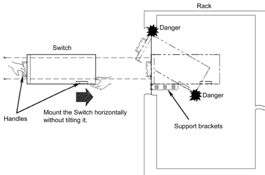
Figure 4-13 Mounting a Switch on the rack
