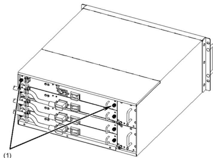
Figure 5-11 Installing a power supply unit (2)
