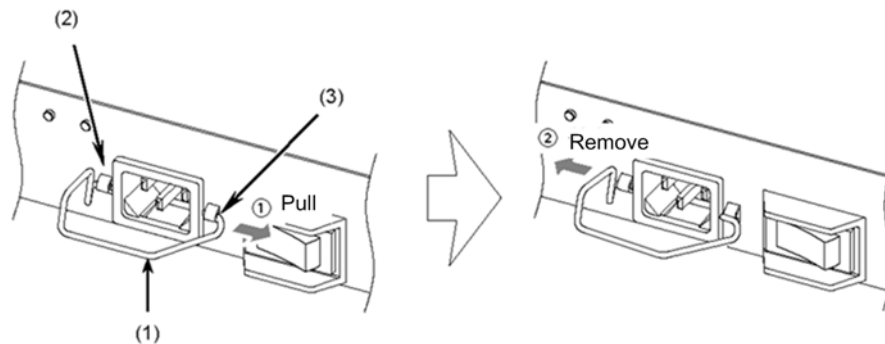
Figure 4-20 Removing the bracket
