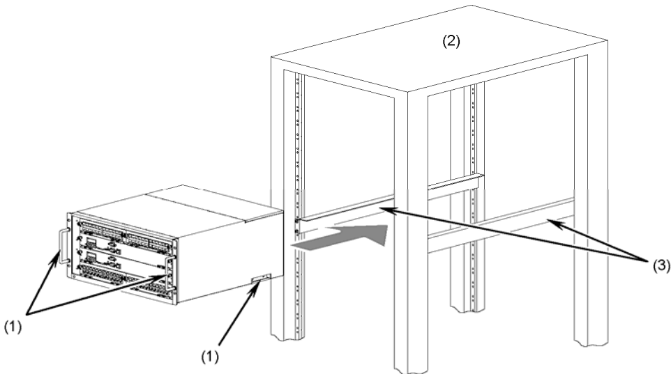
Figure 4-8 Mounting a Switch on the rack
