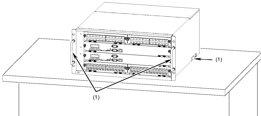
Figure 4-1 Installing a Switch on a desktop
