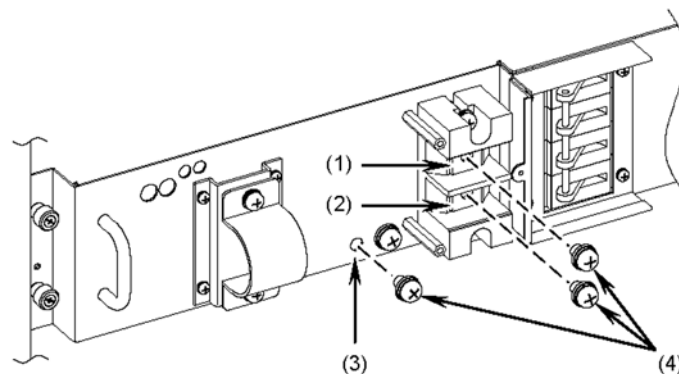
Figure 4-27 Removing the screws
