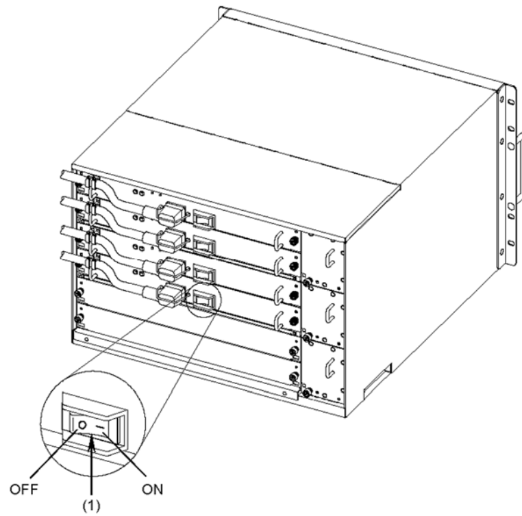
Figure 4-60 Turning off the power
