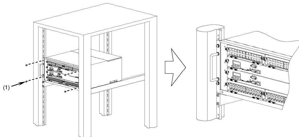
Figure 4-9 Mounting a Switch on the rack
