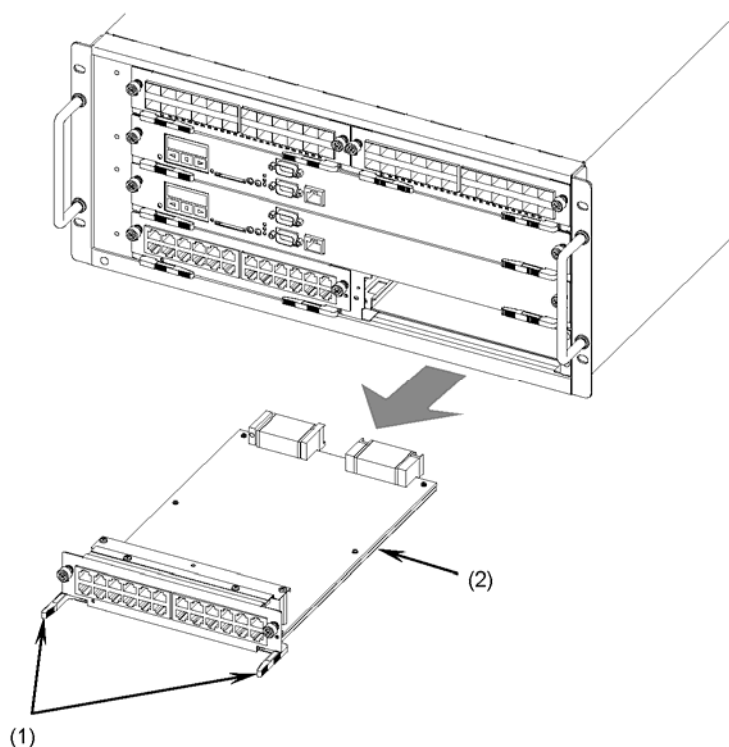
Figure 5-32 Removing a network interface unit (3)
