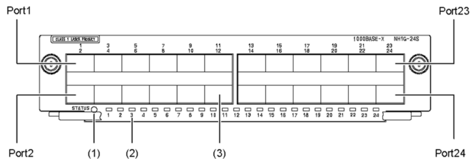
Figure 1-24 Front view
