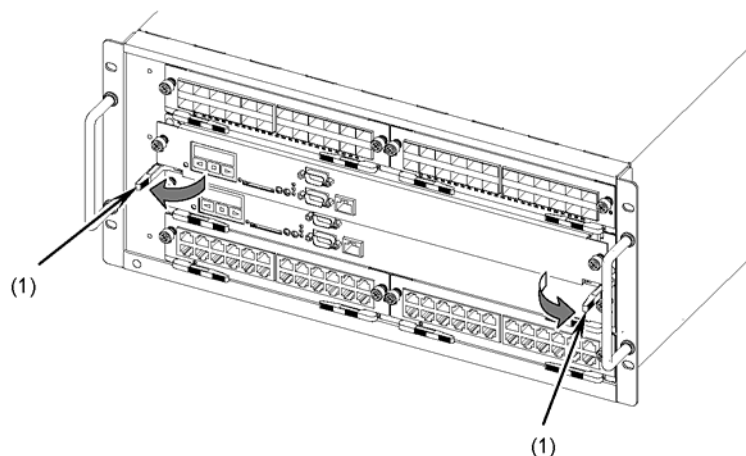
Figure 5-21 Removing a control and switching unit (2)
