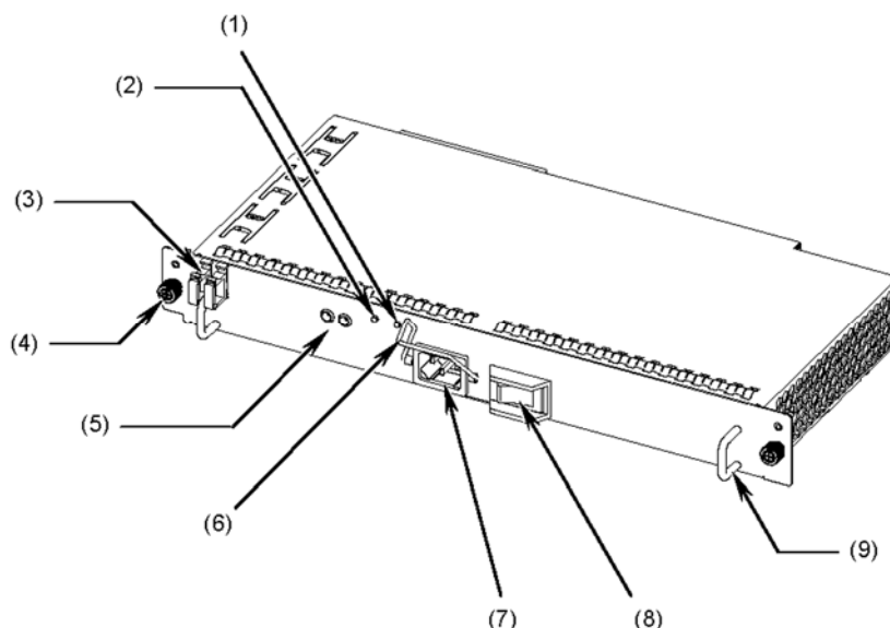
Figure 1-14 External appearance
