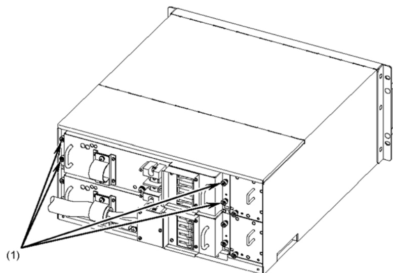
Figure 5-17 Installing a power supply unit (2)
