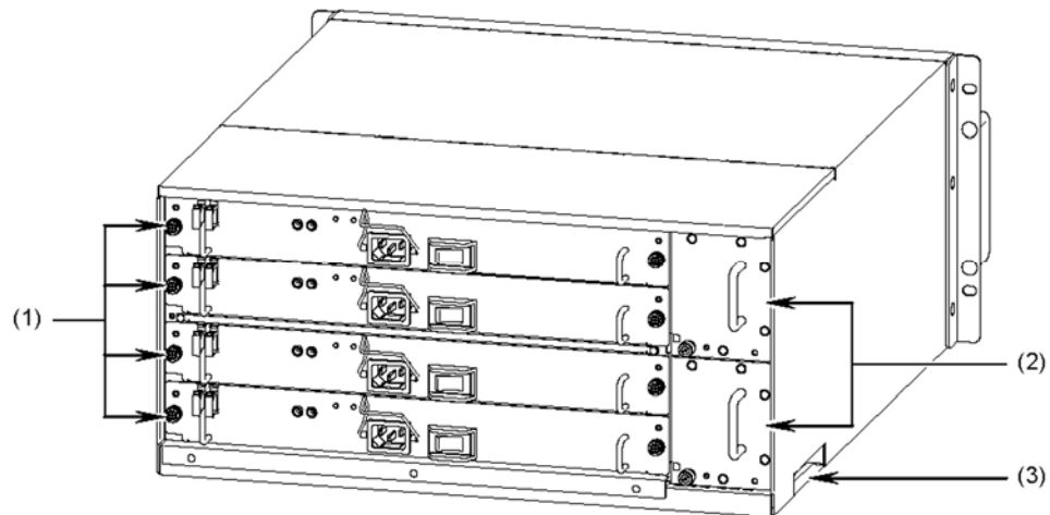
Figure 1-2 Rear view (with an AC power supply unit installed)
