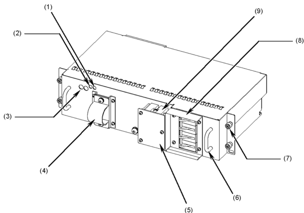
Figure 1-16 External appearance
