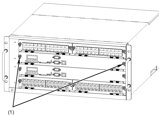
Figure 5-20 Removing a control and switching unit (1)
