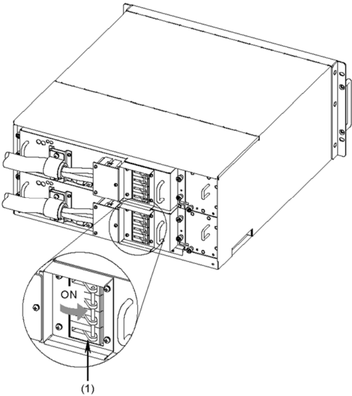
Figure 4-54 Turning on the power
