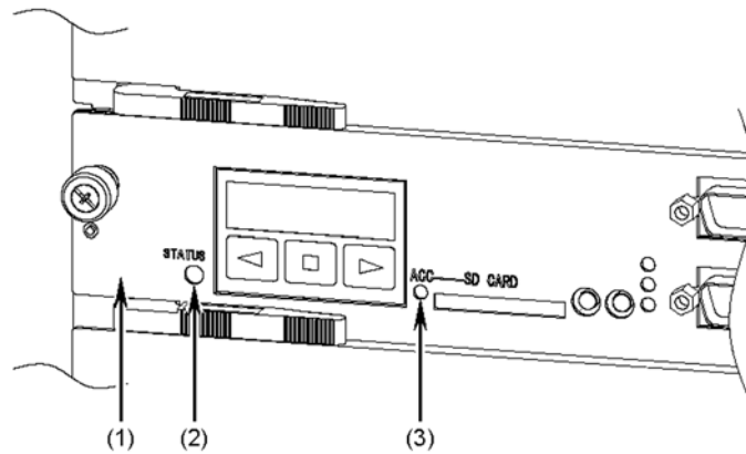
Figure 4-63 Checking the LED
