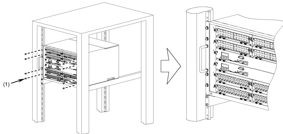
Figure 4-19 Mounting a Switch on the rack
