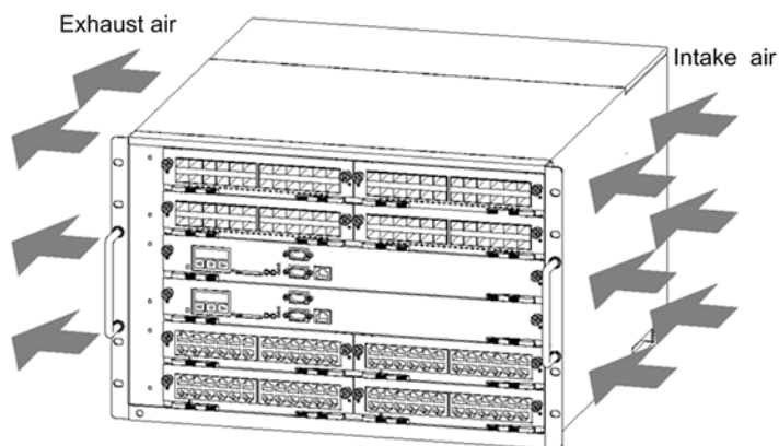
Figure 2-15 AX6608S
