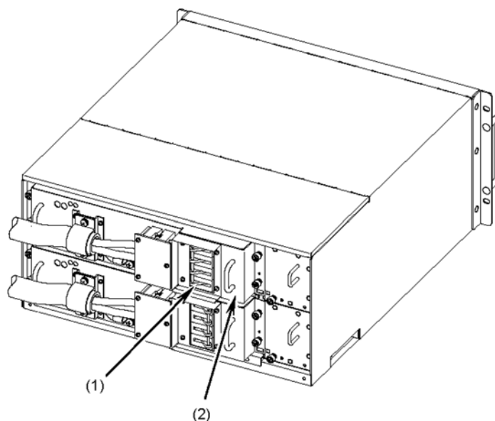
Figure 5-12 Turning off the power
