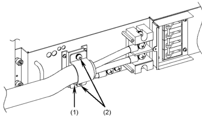
Figure 4-31 Securing the DC power cable
