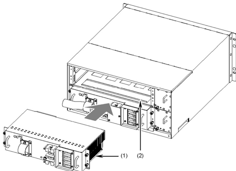
Figure 5-16 Installing a power supply unit (1)
