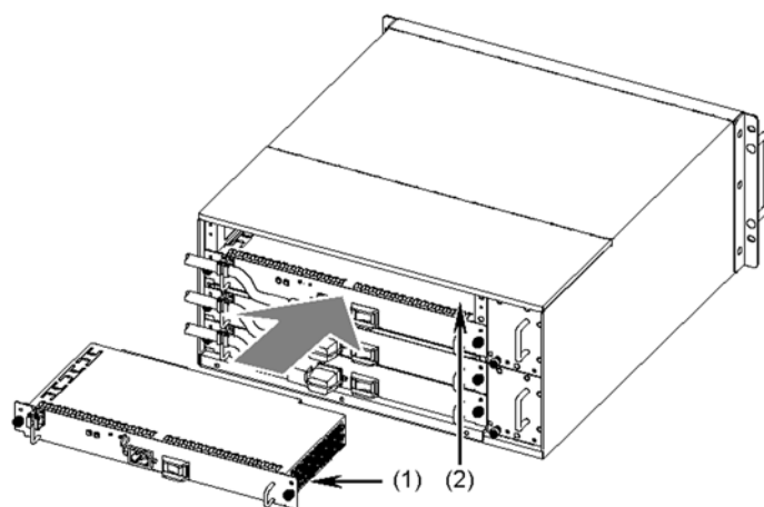
Figure 5-10 Installing a power supply unit (1)
