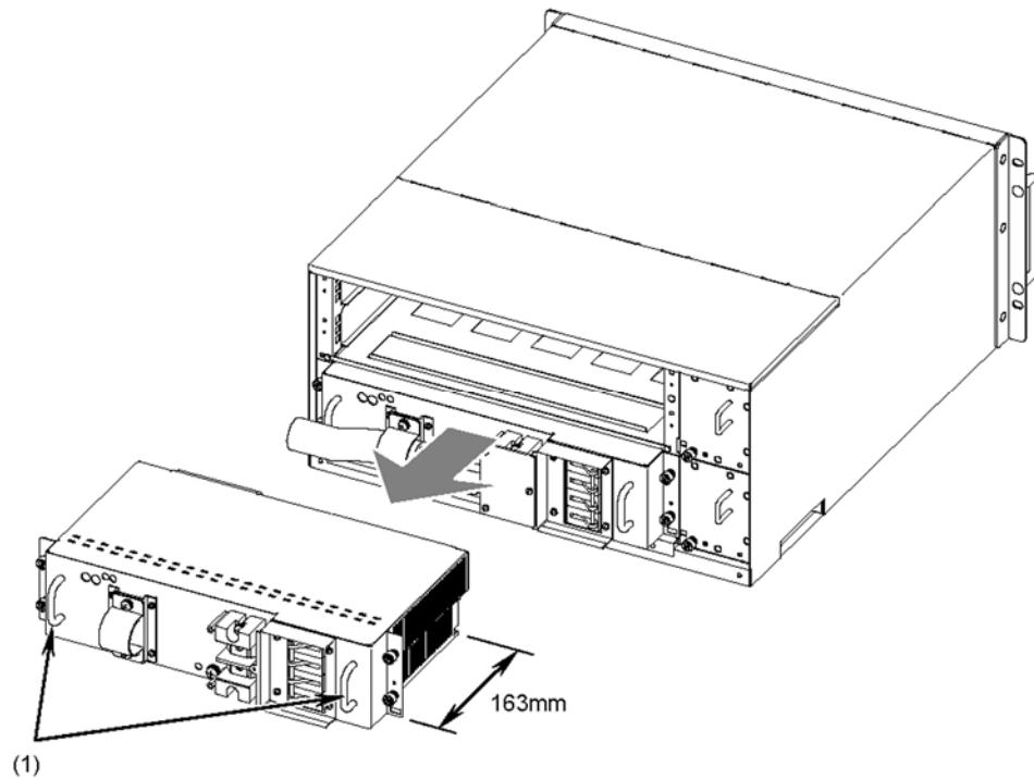
Figure 5-15 Removing a power supply unit (2)
