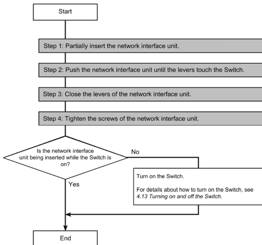
Figure 5-33 Installation overview
