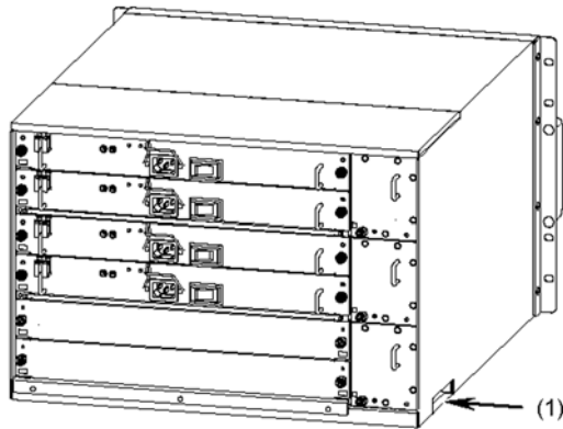
Figure 2-5 Location of handles for the AX6608S (rear)
