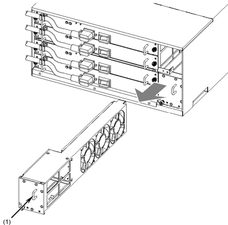
Figure 5-3 Removing a fan unit (3)
