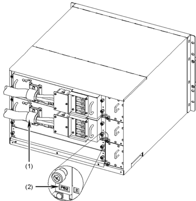
Figure 4-61 Checking the installation location of the power supply unit
