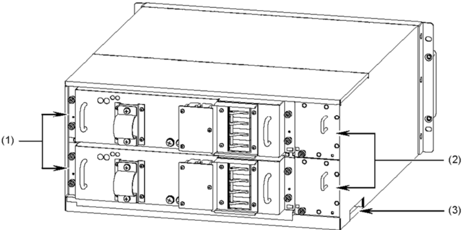
Figure 1-3 Rear view (with a DC power supply unit installed)
