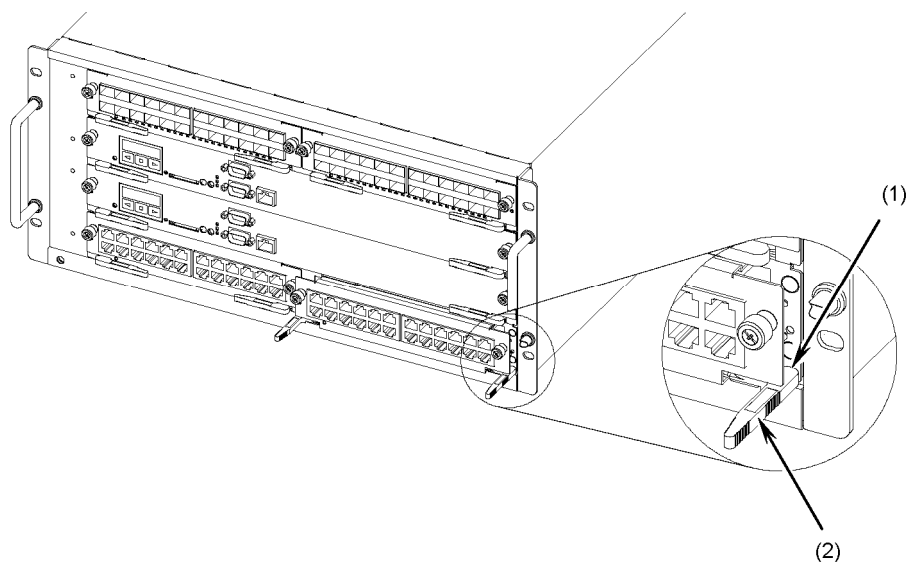
Figure 5-35 Installing a network interface unit (2)
