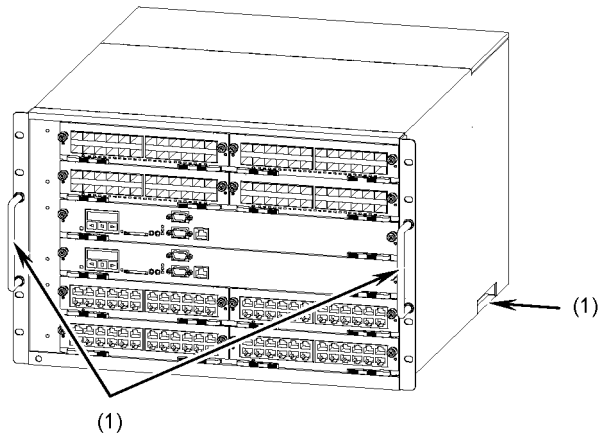
Figure 2-4 Location of handles for the AX6608S (front)
