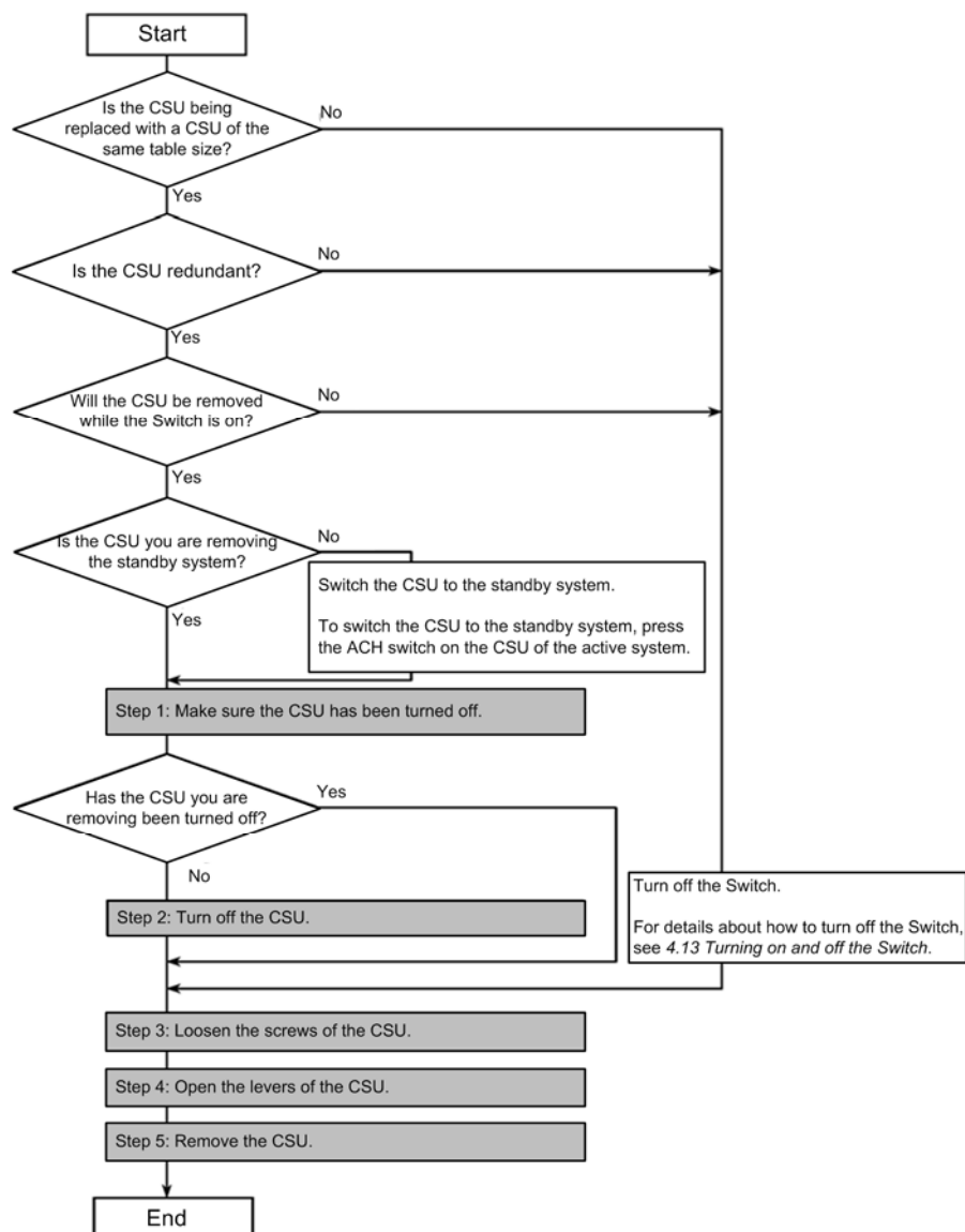
Figure 5-18 Overview of removing a control and switching unit
