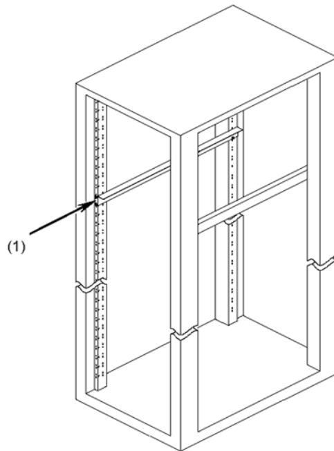
Figure 4-16 Installing a guide rail
