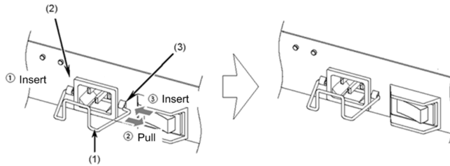
Figure 4-21 Attaching the bracket
