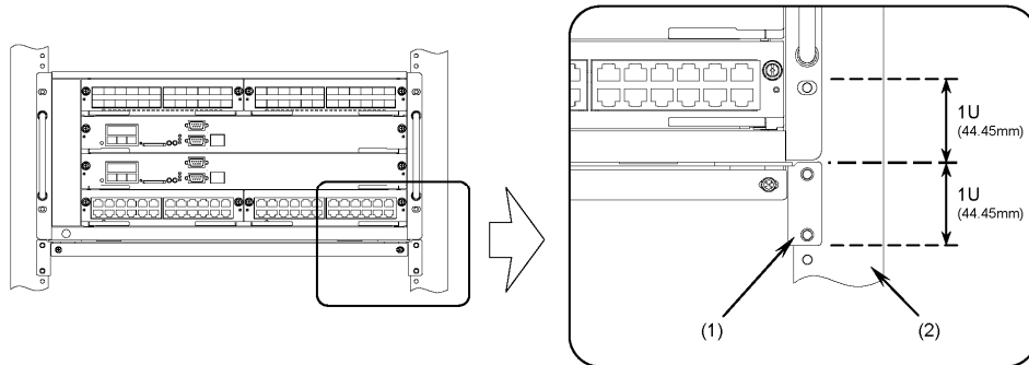
Figure 4-11 Installation location of the support brackets
