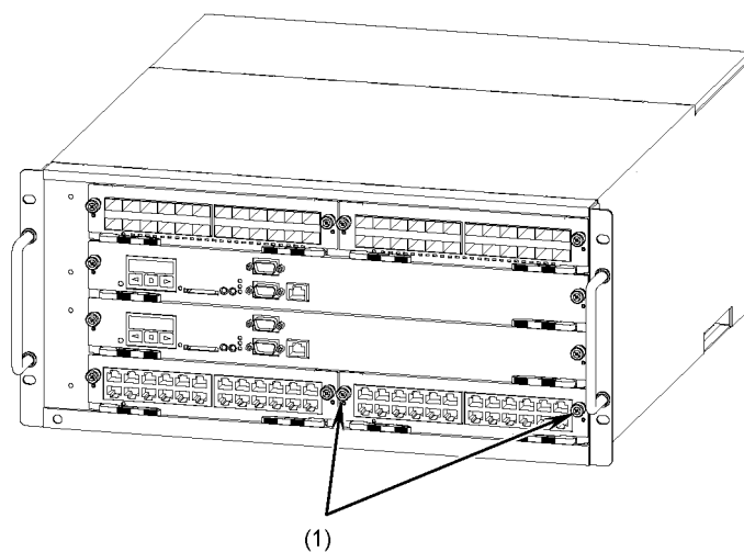
Figure 5-30 Removing a network interface unit (1)
