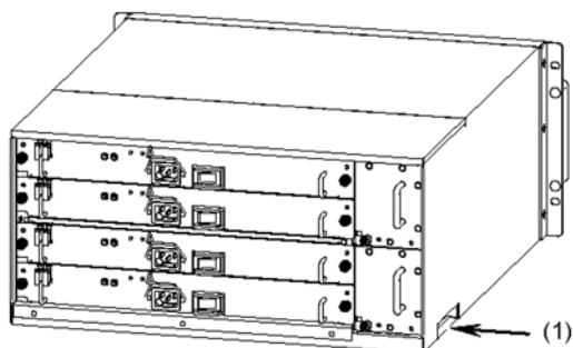
Figure 2-3 Location of handles for the AX6604S (rear)
