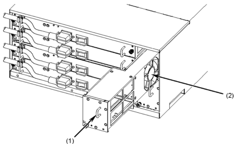
Figure 5-2 Removing a fan unit (2)
