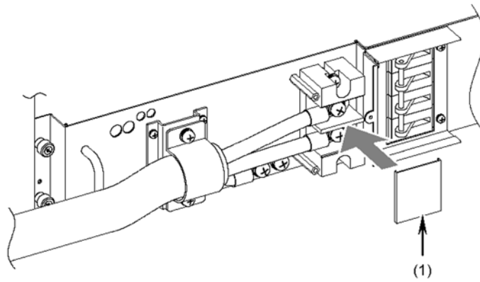
Figure 4-32 Attaching the terminal cover
